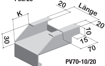
Putzbord P30/20
